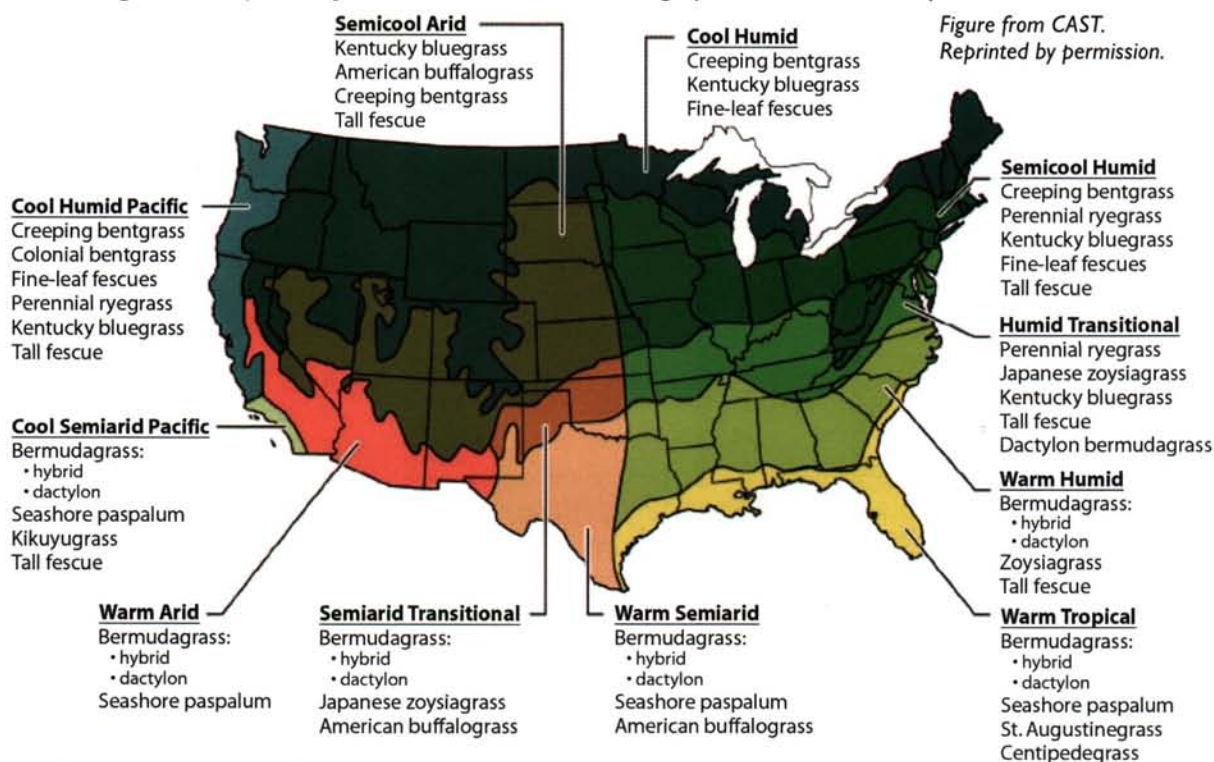
Figure 2: Major Turfgrass Climatic Zones and Geographic Distribution of Species in the U.S.
