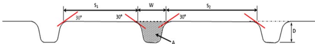
Figure 2: Groove parameters to be measured from the groove profile.
