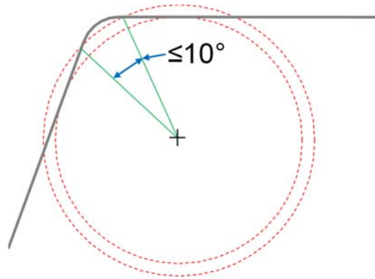
Figure 5: Maximum angular extent of edge protrusion determined by the angle of protrusion
