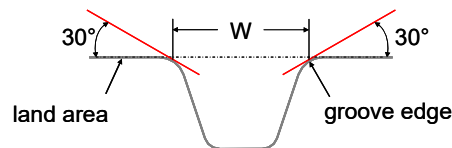
Figure 1: The 30° method for determining the edge points of a groove.
