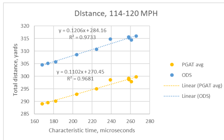
Figure 4: Distance for player groups at 114-120 MPH clubhead speed (PGA TOUR average and Overall Distance Standard). Note that correlation to characteristic time is particularly strong.
